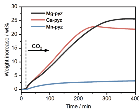
Fig. 2 Isothermal TGA profiles of M-pyz ( M = Mg^{2+} , Ca^{2+} , Mn^{2+} ) under CO_2 flow (0.1 MPa, 30 mL min -1 ) at 40 °C.
