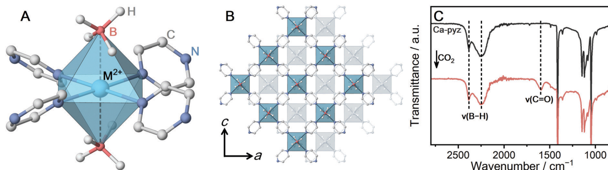
Fig. 1 (A) Local coordination geometry of M-pyz ( M = Mg^{2+} , Ca^{2+} , Mn^{2+} ). (B) ABAB stacking structure of the extended 2D layers of M-pyz ( M = Mg^{2+} , Ca^{2+} , Mn^{2+} ). (C) IR spectra of Ca-pyz before and after CO_2 adsorption at 25 °C.
