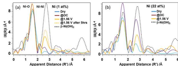
Fig. 3 Ni EXAFS spectra acquired under dry, OC potential and OER potential (+1.56 V) conditions using (a) 1% Ni ( \beta -FeOOH:Ni) and (b) 22% Ni ( \beta -FeOOH:Ni) surface-decorated with \text{Ni}(\text{OH})_2 together with that of the reference compound \beta -Ni(OH) _2 .
