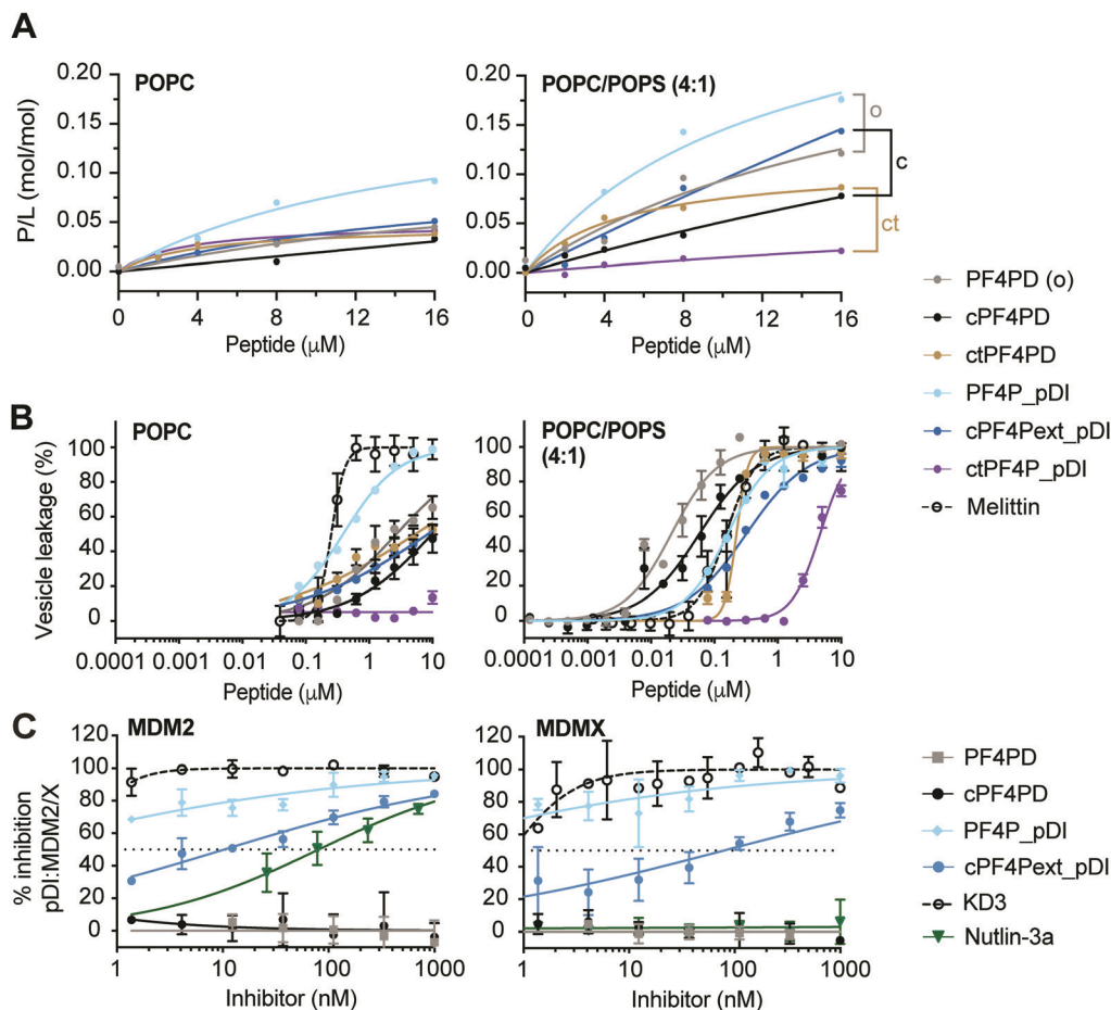
Fig. 3 Grafted peptides bind and lyse model membranes with PS-headgroups and also inhibit pDI:MDM2/X interactions. (A) Binding of peptide to neutral (POPC) and anionic (POPC/POPS, 4 : 1) phospholipid bilayers. Peptides were injected over lipid bilayers on an L1 chip at varying concentrations and peptide-to-lipid ratio (P/L) was determined at the end of the association phase (170 s) when peptide–lipid binding reached a plateau (see Fig. S5, ESI†). Grafted peptides were compared to the parent peptide according to their format: o, open; c, disulfide cyclized; ct, thioether cyclized, by considering relative differences in P/L for 2–16 \mu\text{M} peptide. (B) Membrane leakage induced by peptides. Peptides at varying concentrations were incubated with vesicles (lipid concentration at 5 \mu\text{M} ) loaded with self-quenching concentrations of carboxyfluorescein (CF); the percentage of vesicles with their membrane disrupted was determined by measuring the fluorescence emission intensity of CF released ( \lambda_{exc} = 485 \text{ nm}/\lambda_{em} = 520 \text{ nm} ). 100% of vesicles with leaky membranes was established using 0.1% (v/v) Triton X-100. Melittin, a membrane-disruptive peptide, was included as a positive control. Data points and \text{LC}_{50} values are mean \pm SD from at least two technical replicates from the same experiment. (C) Inhibition pDI:MDM2 and pDI:MDMX interactions by cPF4PD and analogues. FITC-labeled pDI (F-pDI) was used as a p53 mimetic and inhibition of binding to MDM2 and MDMX was determined by measuring the variation in fluorescence polarization of F-pDI. The fluorescence polarization of free F-pDI was used to define 100% inhibition of pDI:MDM2/X interactions, and the fluorescence polarization obtained with pDI:MDM2/X was used to define 0% of inhibition. Controls included: KD3, a lactam-stabilized pDI peptide with high affinity for MDM2 and MDMX; and Nutlin-3a, a small molecule with high affinity for MDM2 but not MDMX. The inhibitor concentration required to inhibit 50% of F-pDI:MDM2/X interactions ( \text{IC}_{50} ) was determined from the dose response curves. Data points are mean \pm SD from three technical replicates from the same experiment.
