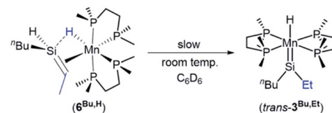
Scheme 4 Solution decomposition of [(\text{dmpe})_2\text{MnH}(\text{}^n\text{BuHSi}=\text{CHMe})] ( 6^{\text{Bu,H}} ) to form silylene complex \text{trans}-[(\text{dmpe})_2\text{MnH}(\text{SiEt}^n\text{Bu})] ( \text{trans-}3^{\text{Bu,Et}} ) as the major product.
