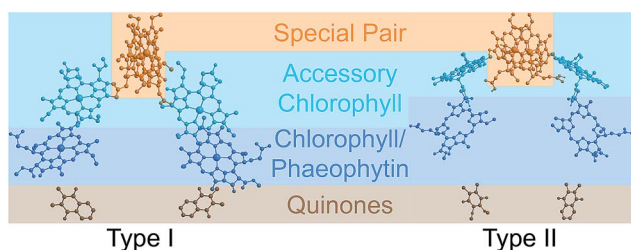
Fig. 1 Photosynthetic reaction centres (RCs). All extant RCs are dimeric, comprising special pair chlorophylls, accessory chlorophylls, secondary chlorophylls or bacteriopheophytin, and quinones. Bacteria use bacteriochlorophyll and bacteriopheophytin instead. Shown are crystallographic structures, 9,10 with chlorophyll tails and supporting protein removed for clarity.
