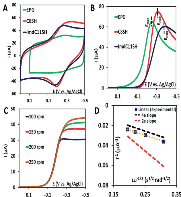
Fig. 3 (A) CV data of Fe III Cl–MARG over the EPG electrode (green), C_8SH SAM- (red) and ImdC 11 SH SAM (blue) modified Au electrodes in the absence of O 2 in pH 7 phosphate buffer with KPF 6 supporting electrolyte at a scan rate of 1 V s -1 ; (B) LSV data of the complex in air saturated pH 7 phosphate buffer over EPG (green), C_8SH SAM (red) and ImdC 11 SH SAM (blue) at 0 rpm at a scan rate of 50 mV s -1 ; (C) RDE plots of the catalyst over the EPG electrode for multiple rotations at a scan rate of 50 mV s -1 ; (D) K–L plot of the catalyst at a potential of –0.5 V.
