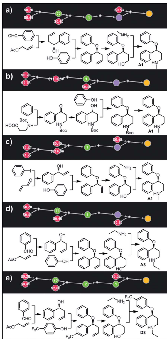
Fig. 5 Top-scoring solutions proposed by Chematica for the synthesis of individual members of the fluoxetine library: (a–c) target A1 , (d) target A3 , and (e) target D3 . Node coloring scheme is as in Fig. 4. For raw Chematica output and synthetic details, see Fig. S5–S7.†
