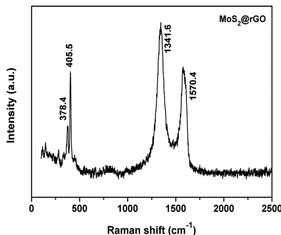
Fig. 2 Raman spectrum of MoS 2 @rGO composite.
