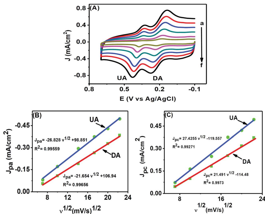
Fig. 8 (A) CVs of 50 \mu\text{M} DA and 200 \mu\text{M} UA at the PTPCNs/GCE in 0.1 M PBS of pH 7.0 at different scan rates (a–f): 50, 100, 200, 300, 400, 500 \text{mV s}^{-1} . The relationship between the oxidation peak current densities (B) and reduction peak current densities (C) of DA and UA with the square root of the scan rates.
