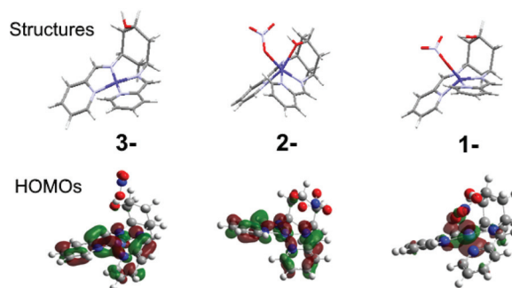
Fig. 2 DFT calculated structures and HOMOs of 2 in its one (1-), two (2-) and three (3-) electron reduced states.
