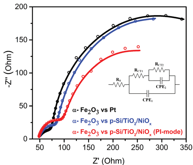
Fig. 4 Nyquist plots of \alpha\text{-Fe}_2\text{O}_3 vs. Pt or p-Si/TiO 2 /NiO x in 1 M NaOH (pH 13.8) under standard (1 sun) single or parallel illumination (PI-mode). The inset shows the equivalent circuit 30 employed for analyzing the Nyquist plots. The fit data are provided in ESI Table S2.†
