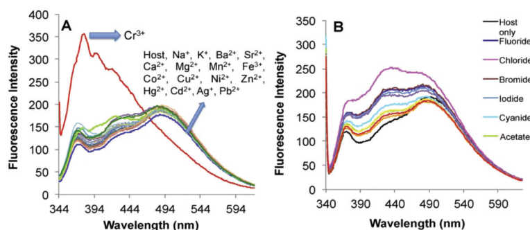
Fig. 9 Changes in the fluorescence spectrum of 10 (FONs) ( 20 \text{ M} ) in aqueous medium upon the (A) addition of 50 \text{ M} of a particular metal nitrate salt in an aqueous medium and (B) addition of 50 \text{ M} of a particular anion as tetrabutylammonium salt in an aqueous medium. Adapted with permission from ref. 32. Copyright 2015 Elsevier Ltd.
