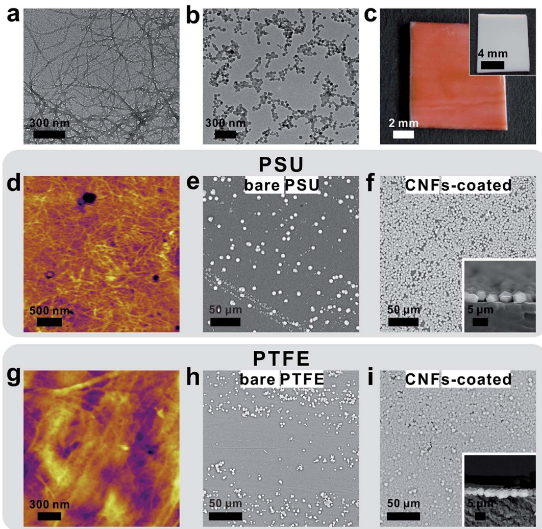
Fig. 1 TEM images of CNFs (a) before and (b) after ZIF-8 mineralization. (c) The photograph of a CNFs-PTFE plate stained by Congo red (inset: the photograph of a bare PTFE plate stained by Congo red). AFM images of CNFs deposited on (d) PSU and (g) PTFE. SEM images of ZIF-8 particles grown on (e) bare PSU, (h) bare PTFE, (f) CNFs-PSU and (i) CNFs-PTFE. Insets in (f) and (i) are the cross-section SEM images of the corresponding samples.
