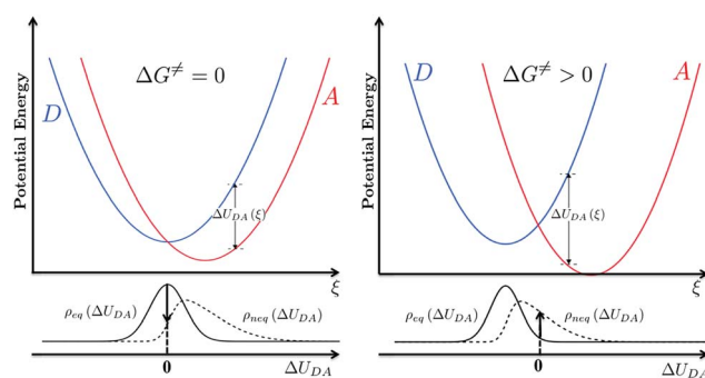
Fig. 6 IVR induced change to the probability density of energy gaps near the DA surface crossing associated with a classical reaction coordinate. \Delta U_{DA}(\xi) is the donor-acceptor energy gap as a function of reaction coordinate \xi . \rho_{eq}(\Delta U_{DA}) is the density of state as a function of \Delta U_{DA} at thermal equilibrium ( \rho_{eq}(\Delta U_{DA}) = \frac{1}{\sqrt{2\pi}(\hbar/\tau_{FC})} \exp \left[ -\frac{(\Delta U_{DA} - (\Delta G + \lambda))^2}{4(\hbar/\tau_{FC})^2} \right] ). IVR excitation of classical reaction coordinates produces a non-equilibrium density of states ( \rho_{neq}(\Delta U_{DA}) ). For an activationless reaction (left, \Delta G = 0 ), a more rapidly decaying energy gap correlation function induced by IVR would deplete population from the curve crossing region and lead to a decrease in the ET rate. For an activated ET reaction (right, \Delta G > 0 ), more rapid fluctuations of the energy gap may increase the population near the curve crossing and effectively enhance the ET rate.
