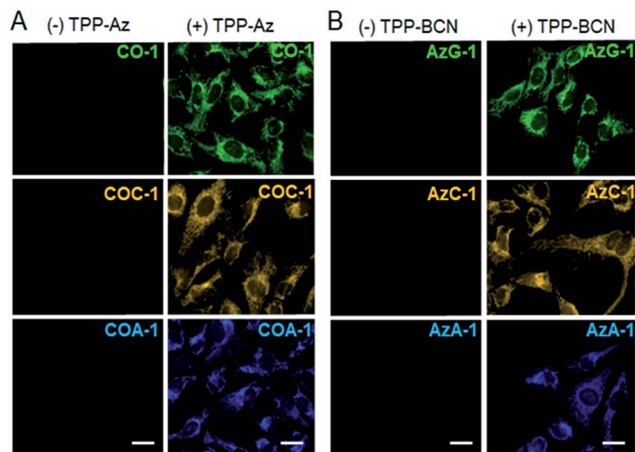
Fig. 2 Fluorescence imaging of mitochondria in live U-2 OS cells labelled with: (A) COA-1, COC-1, and COA-1 in the absence and presence of TPP-Az, and (B) AzG-1, AzC-1 and AzA-1 in the absence and presence of TPP-BCN. The probes were observed to be washed out of the cells in the absence of reporter, while specific labelling of the mitochondria was observed out of a low background in cells pre-treated with reporter. The scale bar is 20 \mu\text{m} .
