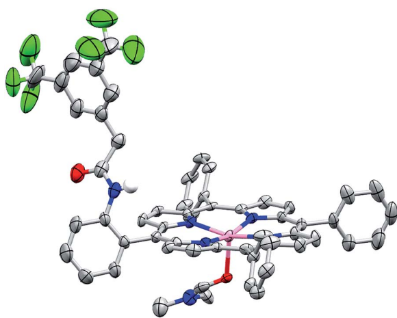
Fig. 2 Solid-state structure of Zn- ortho -1-amide. Non-coordinated solvent molecules and non-amide hydrogen atoms have been omitted for clarity. Thermal ellipsoids are shown at the 50% level.
