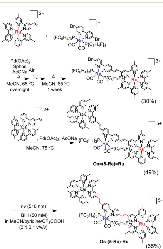
Scheme 3 Synthesis of Os-(5-Re)-Ru .
