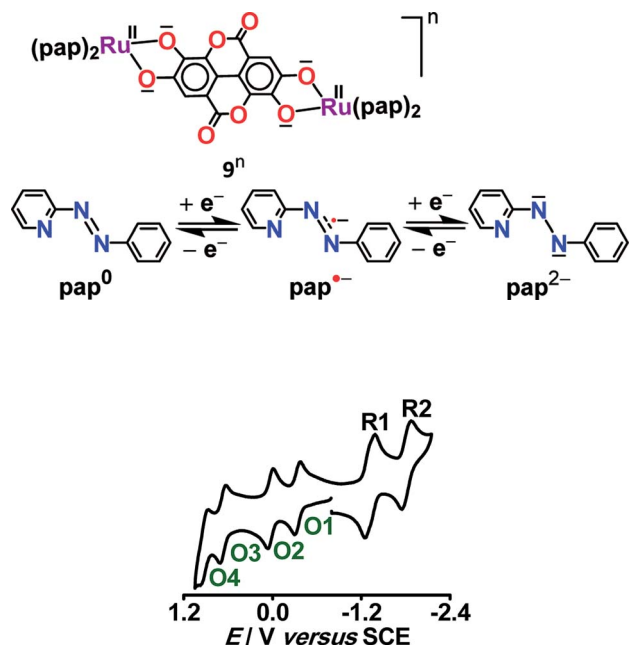
Fig. 8 Cyclic voltammograms of 9 in \text{CH}_3\text{CN} .
