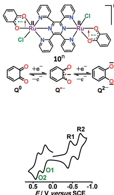
Fig. 10 Cyclic voltammogram of 10 in \text{CH}_3\text{CN} .
