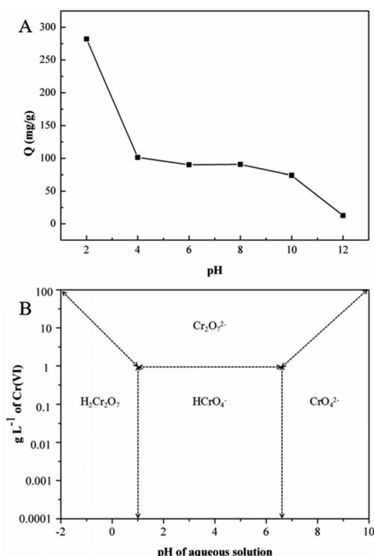
Fig. 5 (A) Effect of pH on the adsorption of \text{Cr}(\text{vi}) by GMFP: temperature, 298.15 \text{ K} ; adsorption time, 6 \text{ h} ; and initial \text{Cr}(\text{vi}) concentration, 300 \text{ mg L}^{-1} , (B) relative distribution of \text{Cr}(\text{vi}) species in water as a function of pH and \text{Cr}(\text{vi}) concentration (adapted from ref. 1).
