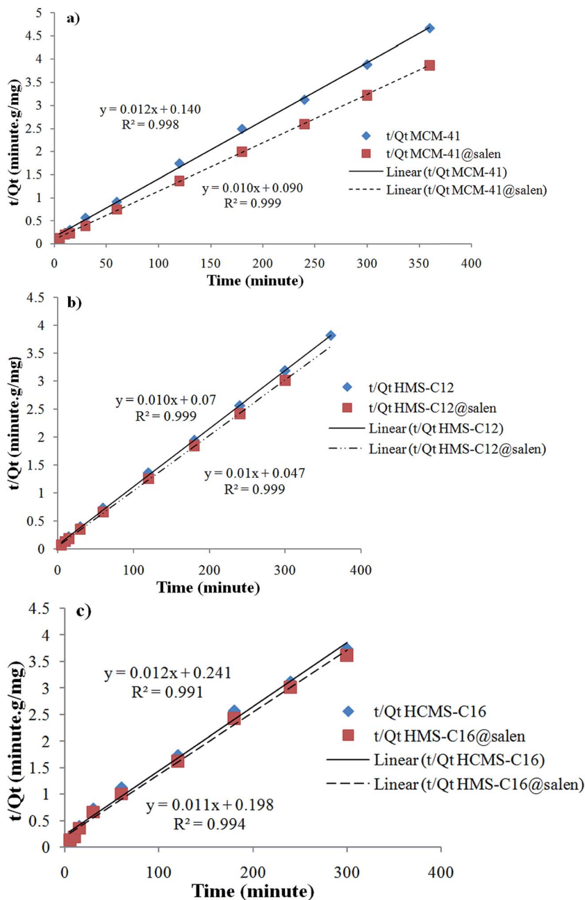
Fig. 14 Pseudo-second order sorption kinetics of Pb(II) onto (a) MCM-41, MCM-41@salen; (b) HMS-C12, HMS-C12@salen; (c) HCMS-C16 and HMS-C16@salen.
