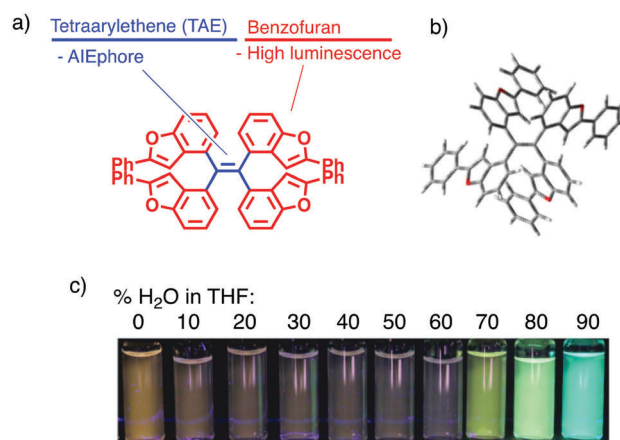
Fig. 1 Tetrakis(benzo[b]furyl)ethene ( TBFE ). (a) Molecular design. (b) Crystal structure showing twisting around the TAE centre (see ESI†). (c) Fluorescence intensity dependent on THF/H 2 O ratio (excitation at 365 nm).
