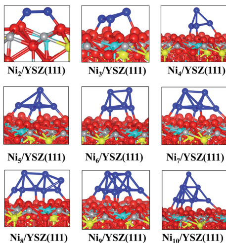
Fig. 4 Side views of the most stable configurations of Ni n /YSZ(111) systems. Colour key: red, grey, blue and cyan spheres correspond to oxygen, Zr, Ni and Y atoms, respectively. The oxygen vacancy is represented by a yellow sphere.
