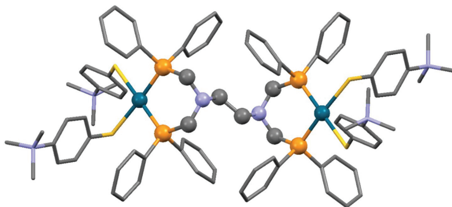
Fig. 9 X-Ray structure of [\text{Pd}(\text{tab})_2]_2(\mu\text{-dppda})\text{Cl}_4 [CCDC 800046]. 75
