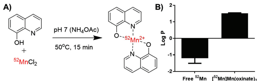
Fig. 2 (A) Radiochemical scheme for the synthesis of [\text{Mn}^{52}\text{Mn}(\text{oxinate})_2] , and (B) chart showing the \log P values of unchelated ^{52}\text{Mn} and [\text{Mn}^{52}\text{Mn}(\text{oxinate})_2] in water/octanol. Error bars represent standard deviation ( n = 2 ).
