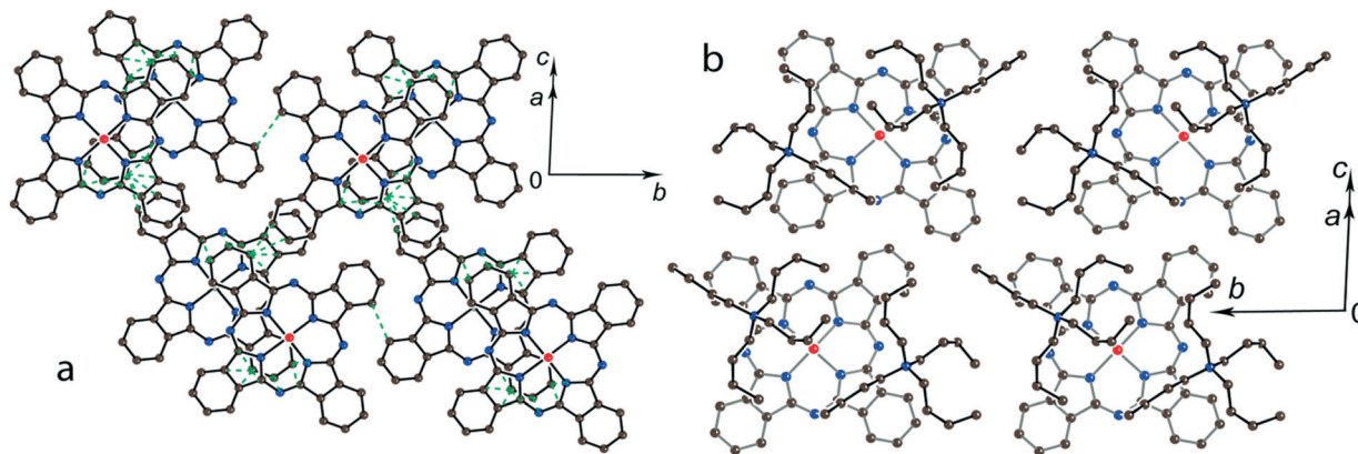
Fig. 3 (a) View of the phthalocyanine layer composed of the \pi -stacking [\text{Ti}^{\text{IV}}\text{O}(\text{Pc}^{3-})]_2 dimers in 2 . 12 Short van der Waals C...C contacts are shown by green dashed lines. (b) Projection of the \text{Bu}_4\text{N}^+ layer on the phthalocyanine layer. Only one phthalocyanine from the dimer is shown (bonds are shown in grey).
