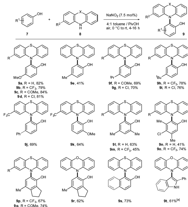
Scheme 3 Scope for the cross-dehydrogenative C–H bond amination. Reaction conditions: 8 (0.2 mmol, 1 equiv.), 9 (3 equiv.), 4: 1 toluene/PivOH (0.05 M), 0 °C to rt under air atmosphere. Yields are given for isolated products after column chromatography. a NOBF 4 (0.02 mmol, 10 mol%) was used as catalyst.
