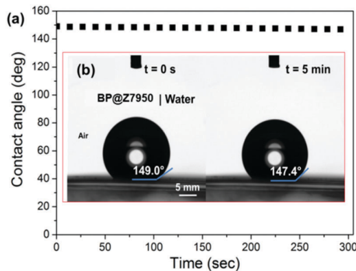
Fig. 4 Contact angle measurements on a PVDF membrane with BP immobilized at the surface. (a) Plot of contact angle ( ^\circ ) over time for a drop of deionized water on the BP supported by PVDF membrane. (b) Optical images (CCD camera) of the contact angle of a deionised water droplet on the BP-coated membrane at t = 0 and 5 min.
