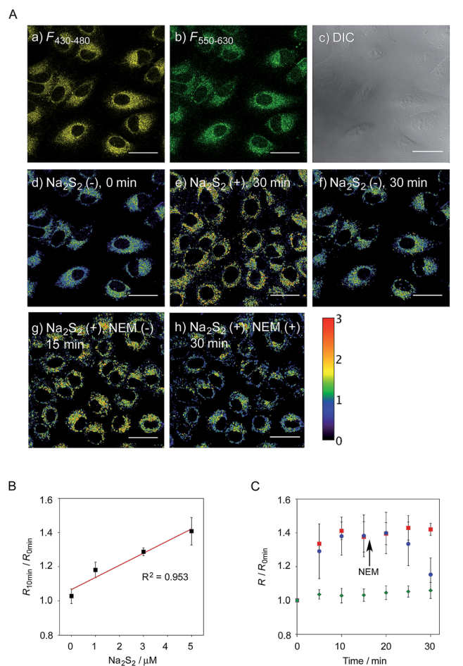
Fig. 4 (A) Fluorescence images of A549 cells treated with 6-AM (5 \mu\text{M} ). (a) F_{430-480} , (b) F_{550-630} , (c) DIC, and (d) ratio image ( R = F_{430-480}/F_{550-630} ). (e) and (f) Ratio image after 30 min in the presence and absence of \text{Na}_2\text{S}_2 (5 \mu\text{M} ), (g) and (h) ratio image after 15 min in the presence \text{Na}_2\text{S}_2 (5 \mu\text{M} ) and subsequent treatment with NEM (100 \mu\text{M} ) for 15 min. Scale bar: 30 \mu\text{m} . (B) Ratio value change of A549 cells upon the addition of various concentrations of \text{Na}_2\text{S}_2 (0–5 \mu\text{M} ), n = 6. (C) Time trace plot of the ratio value in A549 cells upon the treatment with \text{Na}_2\text{S}_2 (5 \mu\text{M} ) (red square, n = 6), \text{Na}_2\text{S}_2 (5 \mu\text{M} ) and the subsequent addition of NEM (100 \mu\text{M} ) at 15 min (blue circle, n = 4), without \text{Na}_2\text{S}_2 and NEM (green diamond, n = 6).
