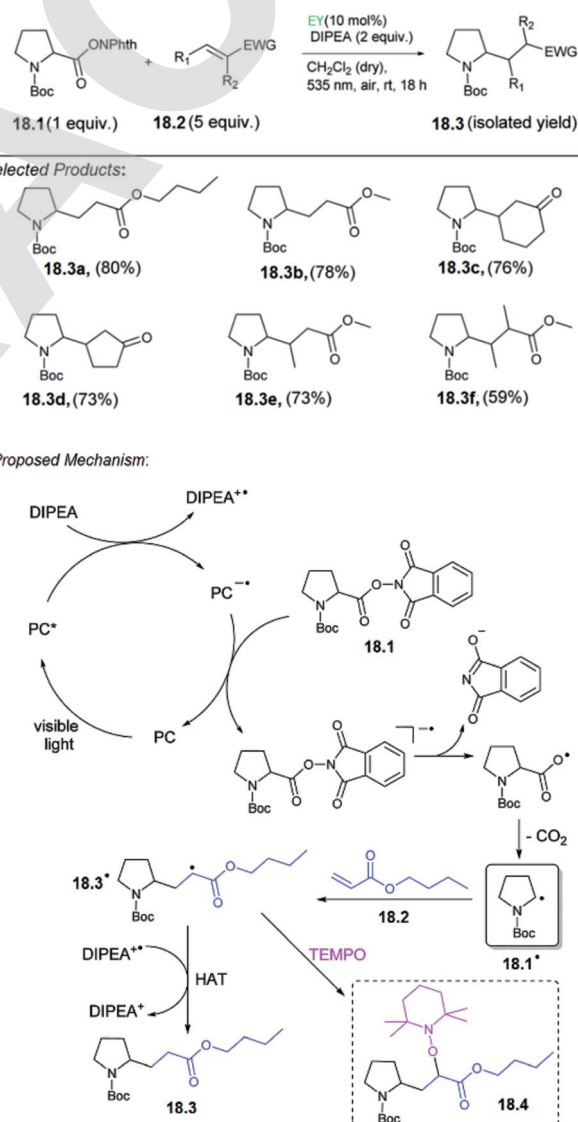
Scheme 18 Decarboxylative alkylation.
