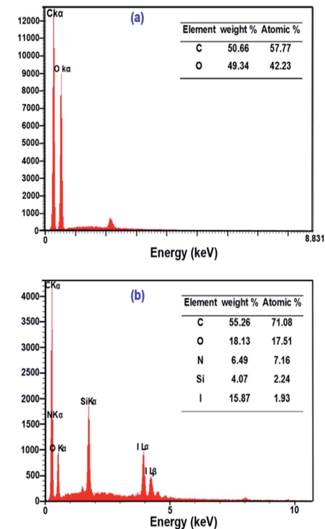
Fig. 4 EDX spectra and tabulated results of neat NFC (a) and NFC 4.0 TMSQI (b).
