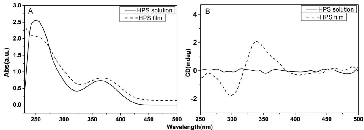
Fig. 1 The UV-vis absorption spectra (A) and CD spectra (B) of HPS in its THF solution (concentration: 10^{-4} M) and at cast film states.
