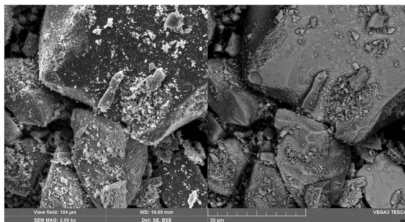
Fig. 4 SEM micrography for a \text{BaTiO}_3:\text{Er}^{3+} 5\%-\text{Yb}^{3+} 1\% sample. Right: Backscattering and Left: secondary electrons.
