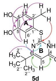
Fig. 5 Important 2 J, 3 J, 4 J and 5 J HMBC correlations of 5d .
