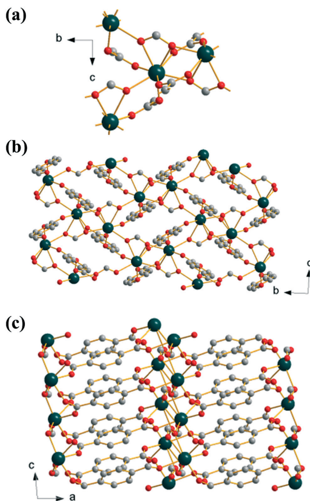
Fig. 3 Structure of (3): (a) local view of the connection of four Yb centres, (b) view along a , and (c) view along b . Atomic labelling scheme is as for Fig. 1 with hydrogen atoms omitted for clarity.
