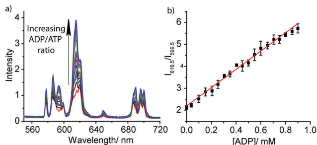
Fig. 3 (a) Ratiometric change in emission spectra of [\text{Eu.1}]^+ (8 \mu\text{M} ) in the presence of increasing ratio of ADP/ATP; (b) plot of the emission intensity ratio, 616.5/599.5 nm, versus mole fraction of ADP. Conditions: buffered aqueous solution (10 mM HEPES, pH 7.0) containing \text{MgCl}_2 (3 mM). Concentration of ADP: 0–0.9 mM, total nucleoside concentration = 1 mM. \lambda_{\text{exc}} = 330 nm, 298 K.
