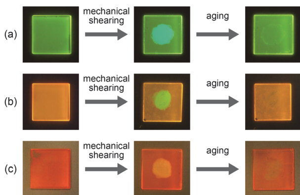
Fig. 4 Luminescence images of compounds 1 (a), 2 (b), and 3 (c) under UV irradiation ( \lambda_{\text{ex}} = 365 \text{ nm} ) before shearing (left), after shearing (center), and after aging at ambient temperature (right). Mechanical shearing is applied to the central part of the sample coated on a quartz substrate.
