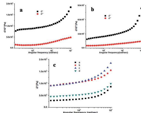
Fig. 4 Mechanical response of the KOH responsive gel of compound 1 in (a) MeOH–water and (b) EtOH–water at 20 °C with small oscillatory shear in the linear viscoelastic regime. (c) Rheological measurements of compound 1 gel with increasing percentage of water in methanol. Water : MeOH for a = 0.5 : 9.5 , b = 0.8 : 9.2 , c = 1 : 9 and d = 1.2 : 8.8 .
