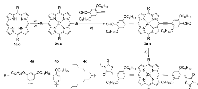
Scheme 1 Synthetic route for 4a-c . Reaction conditions: (a) NBS, CH 2 Cl 2 , pyridine, 0 °C; (b) Zn(AcO) 2 , CHCl 3 , reflux, 4 h; (c) Pd(PPh 3 ) 4 , Cul, Et 3 N, THF, 50 °C, overnight; (d) 3-ethylrhodanine, CHCl 3 , piperidine, reflux, overnight.
