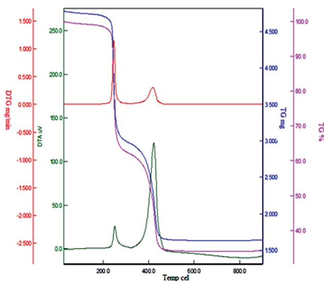
Fig. 4 TGA curve of Cu(II) immobilized on \text{Fe}_3\text{O}_4@SiO_2@L\text{-arginine} .
