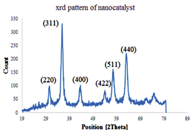
Fig. 3 The X-ray diffraction pattern of Cu(II) immobilized on \text{Fe}_3\text{O}_4@SiO_2@L\text{-arginine} nanoparticle.
