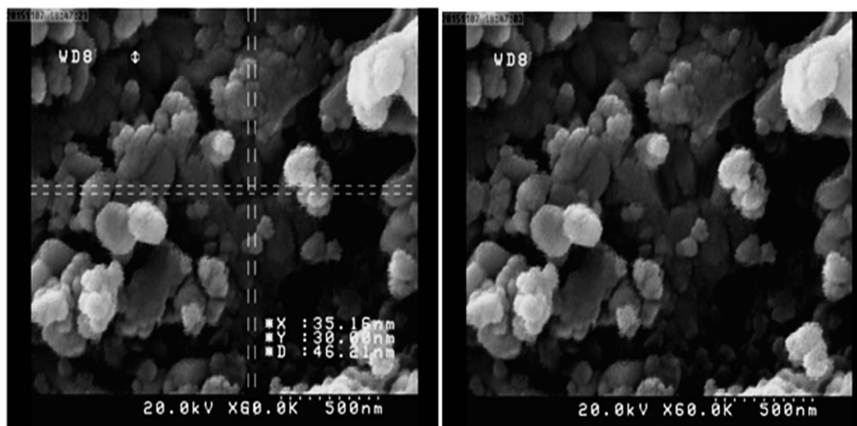
Fig. 2 SEM image of Cu(II) immobilized on \text{Fe}_3\text{O}_4@SiO_2@L\text{-arginine} .
