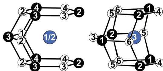
Fig. 4 Coordination environments surrounding the Ce1/2 (left) and Ce3 (right) atoms in the crystal structure of \text{Ce}_3\text{Pt}_4\text{Ge}_6 . Ce atoms are depicted as blue, Pt atoms as black and Ge atoms as open white circles.
