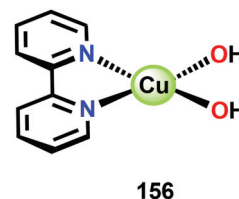
Fig. 51 Structure of the [\text{Cu}(\text{bpy})(\text{OH})_2] complex 156 .
