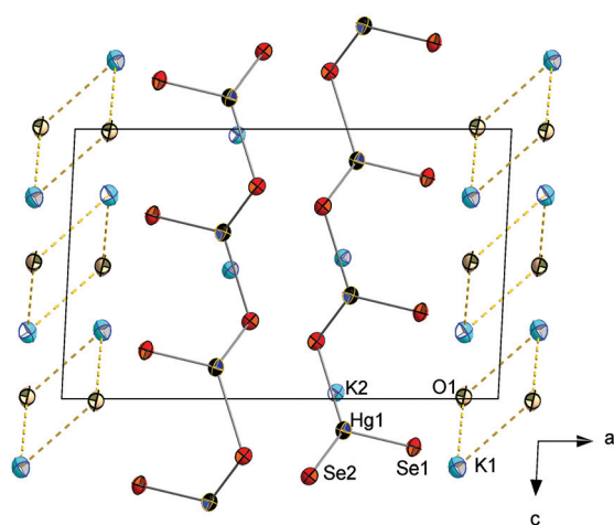
Fig. 4 Fragment of the crystal structure of 4 . Ellipsoids are drawn at 50% probability. Selected structural parameters [ \text{\AA} , ^\circ ]: Hg–Se1: 2.5097(10), Hg–Se2: 2.5908(10)–2.6090(11), K \cdots Se: 3.193(2)–3.497(2), K \cdots O: 2.789(9)–3.426(9), Se–Hg–Se: 107.19(3)–132.38(3).
