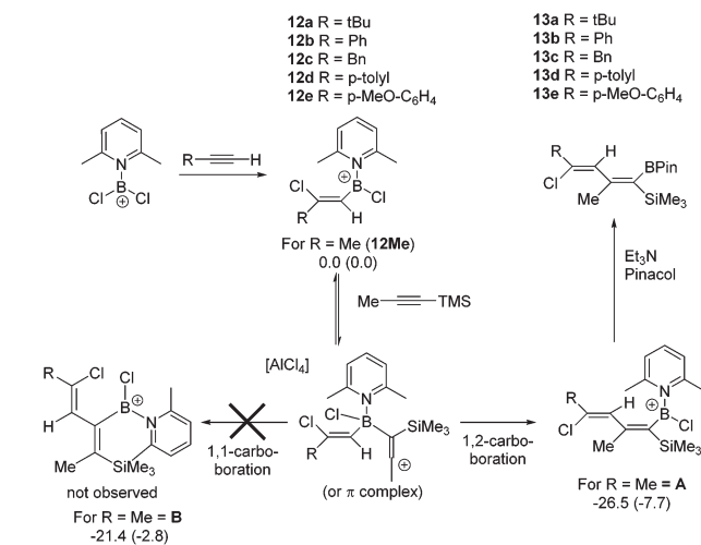
Scheme 4 1-Boradiene formation by haloboration and 1,2-carbaboration. Electronic energies (Gibbs free energies at 293 K) shown in \text{kcal mol}^{-1} for the model system where R = Me (all energies relative to 12Me and 1-TMS-1-propyne at infinite distance).
