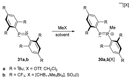
Scheme 10 Diphosphenes 31a,b can only be methylated by very strong methylation agents to form diposphenium cations 30a,b + .
