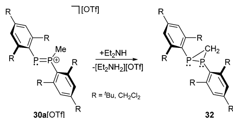
Scheme 11 Formation of diposphenirane 32 by deprotonation of 30a[OTf] .
