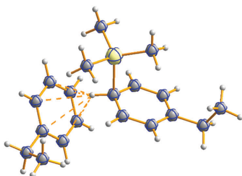
Fig. 41 Molecular structure of [\text{Me}_3\text{Si}(\text{C}_8\text{H}_{10}) \cdot (\text{C}_8\text{H}_{10})]^+ . The weak interaction between the stabilized cation and the adjacent ethylbenzene is indicated by the dashed bonds. M. F. Ibad, P. Langer, A. Schulz and A. Villingner, J. Am. Chem. Soc. , 2011, 133 , 21016–21027. Data from this reference were used to draw this figure.
