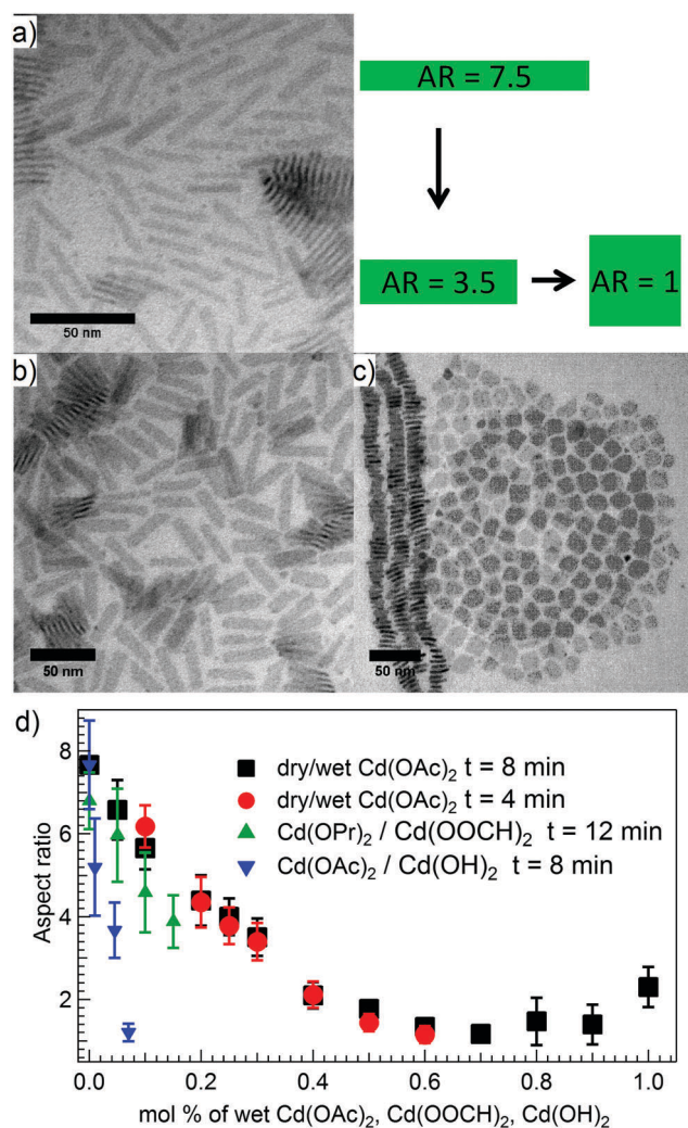
Fig. 2 TEM images of samples (a) NPL-1, (b) NPL-6, (c) and NPL-10 illustrating the aspect ratio control. (d) Plot of the CdSe NPL aspect ratio versus the molar percentage of \text{Cd}(\text{OAc})_2 \cdot 2\text{H}_2\text{O} , \text{Cd}(\text{OOCH})_2 , and \text{Cd}(\text{OH})_2 precursors, respectively.
