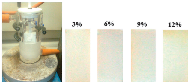
Fig. 1 Camera pictures of cobalt doped ZnS synthesis (left) and thin films deposited onto glass substrates (right) at different concentrations of a cobalt precursor into the chemical bath.
