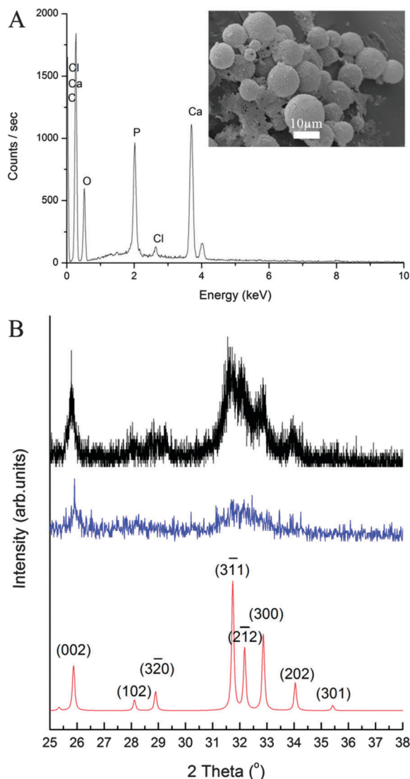
Fig. 4 (A) EDX spectrum and SEM micrograph of CaP capsules. (B) XRD patterns of CaP capsules as synthesized (black line), CaP capsules annealed at 600 °C (blue line), and simulated powder pattern of single crystal hydroxyapatite (red line).
