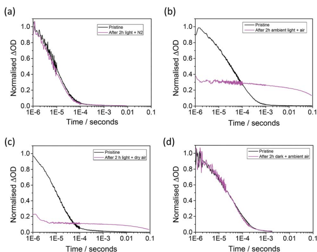
Fig. 4 Effect of exposure to varying environmental conditions for two hours on the transient absorption signal at 1600 nm for a mesoporous \text{Al}_2\text{O}_3 /MAPbI 3 /spiro-OMeTAD film: (a) ambient light, sealed under flowing \text{N}_2 , (b) ambient light, non-sealed, (c) ambient light, sealed under flowing dry air ( \text{H}_2\text{O} < 2 \text{ vpm} ), (d) dark, non-sealed. Laser excitation energy density = 25 \mu\text{J cm}^{-2} at 567 nm.
