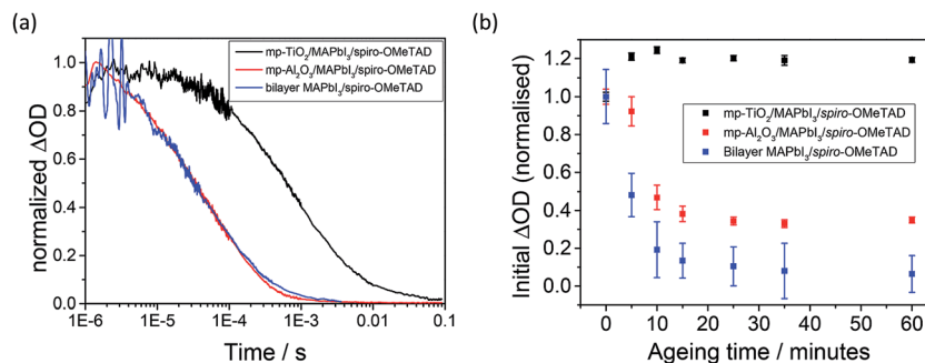
Fig. 3 (a) Time-resolved transient absorption at 1600 nm for pristine mp- \text{TiO}_2 /MAPbI 3 /spiro-OMeTAD (black), mp- \text{Al}_2\text{O}_3 /MAPbI 3 /spiro-OMeTAD (red) and bilayer MAPbI 3 /spiro-OMeTAD (blue) films. All traces normalized to \Delta OD = 1 at 1 \mu\text{s} to highlight differences in recombination kinetics. (b) Relative yield of long-lived charge separation as a function of ageing time in atmospheric conditions under ambient light. Data points determined from the mean amplitude of \Delta OD at 1600 nm between 2 and 5 \mu\text{s} for each measurement. All films were excited at 567 nm with a 25 \mu\text{J cm}^{-2} laser pulse.
