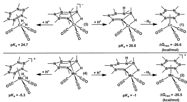
Scheme 4 Calculated \text{pK}_\text{a} values, and free energy of \text{H}_2 loss, for borazine hydride adducts 3 and 4 in \text{Et}_2\text{O} solution.
